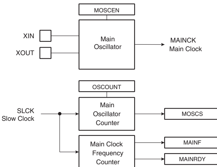
Figure 25-2. Main Oscillator Block Diagram
