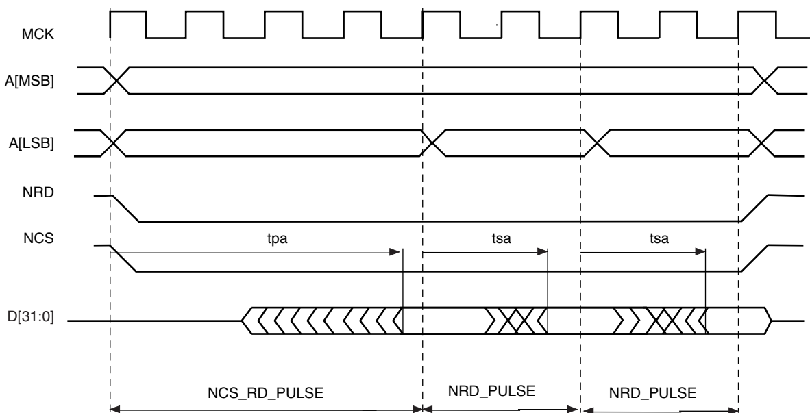
Figure 21-35. Page Mode Read Protocol (Address MSB and LSB are defined in Table 21-7 )
