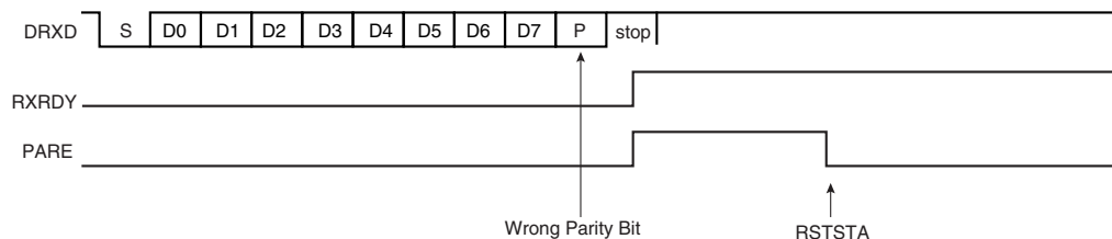
Figure 28-9. Parity Error
