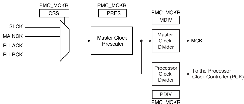
Figure 26-1. Master Clock Controller
