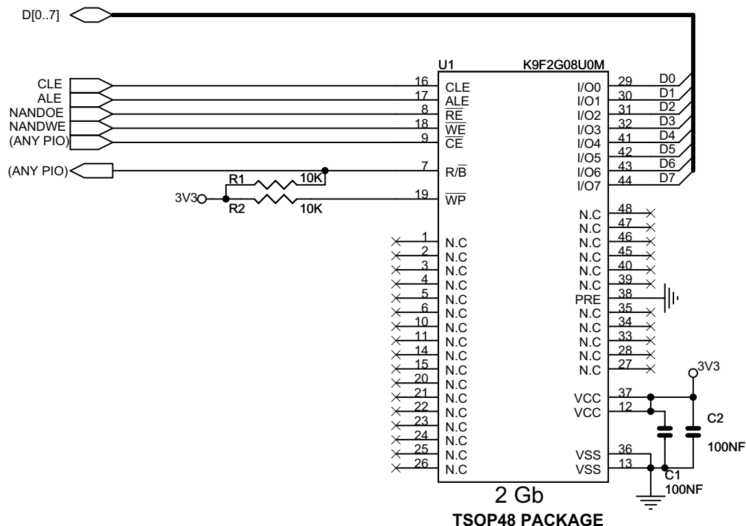
Figure 20-8. Hardware Configuration
