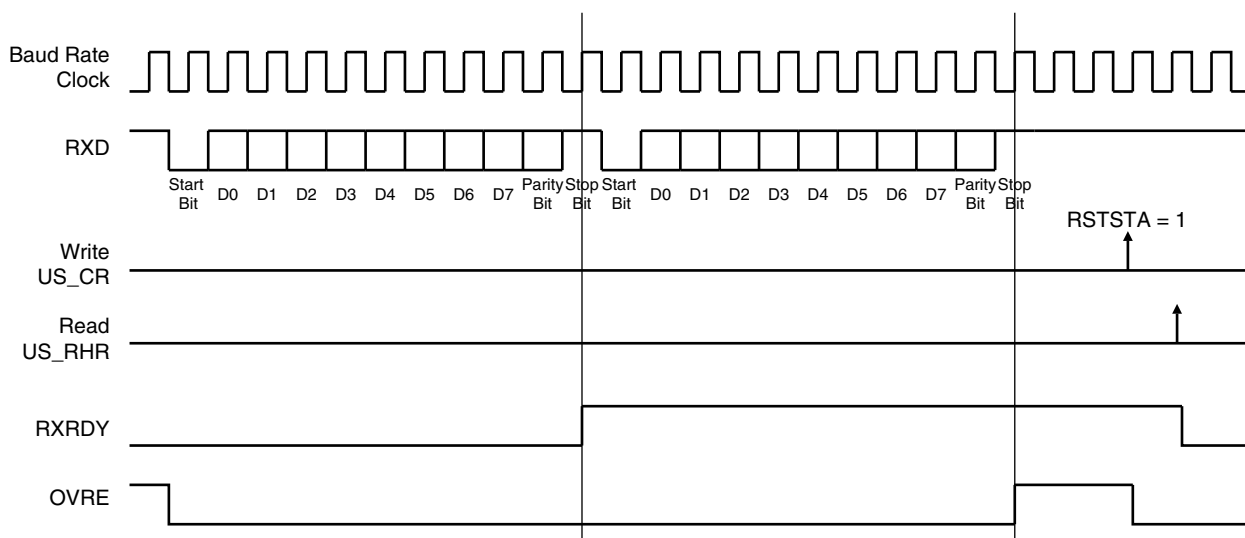
Figure 32-21. Receiver Status
