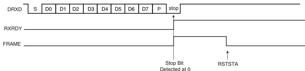
Figure 28-10. Receiver Framing Error
