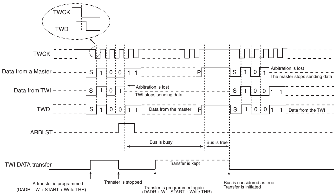
Figure 31-21. Arbitration Cases
