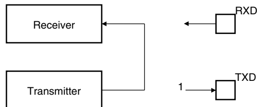
Figure 32-40. Local Loopback Mode Configuration
