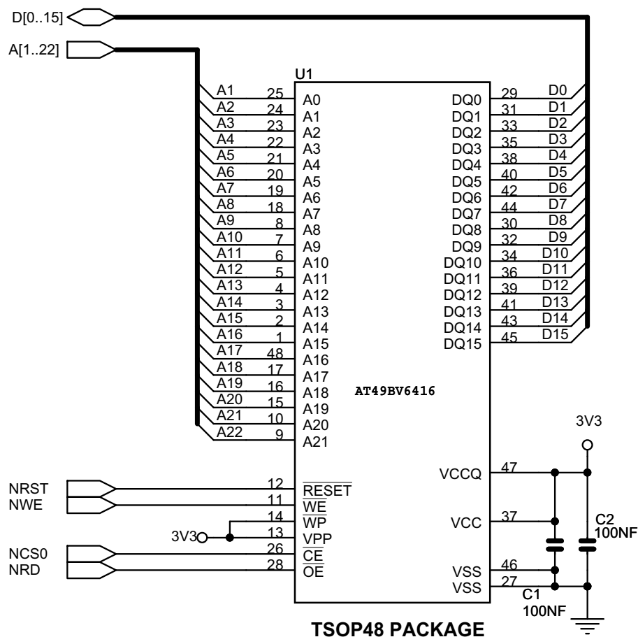
Figure 20-10. Hardware Configuration
