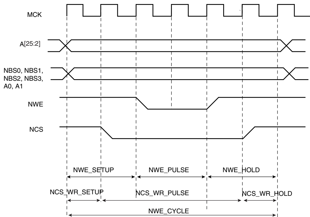
Figure 21-12. Write Cycle
