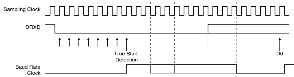
Figure 28-5. Start Bit Detection
