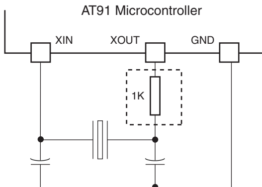
Figure 25-3. Typical Crystal Connection
