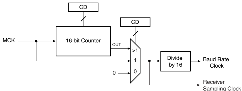
Figure 28-4. Baud Rate Generator
