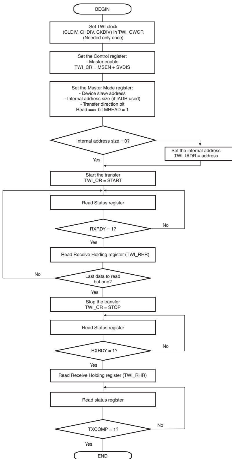
Figure 31-19. TWI Read Operation with Multiple Data Bytes with or without Internal Address
