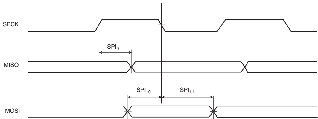
Figure 41-10. SPI Slave Mode with (CPOL = NCPHA = 0) or (CPOL = NCPHA = 1)
