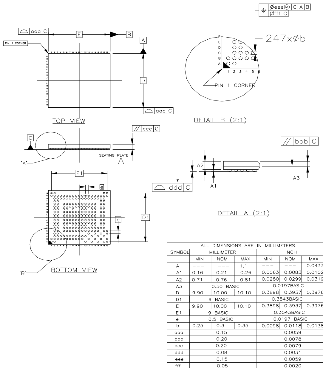
Figure 42-2. 247-ball TFBGA Drawing
