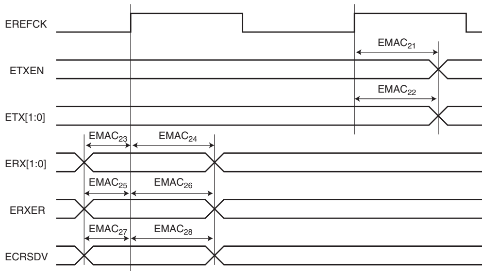
Figure 41-6. EMAC RMII Timings
