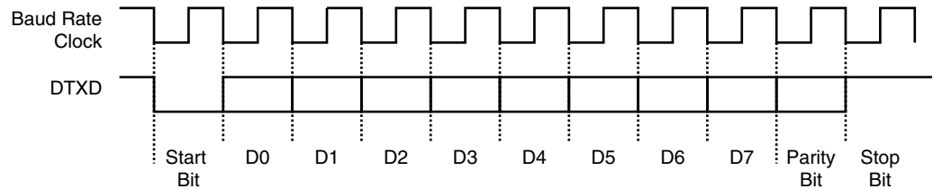
Figure 28-11. Character Transmission
