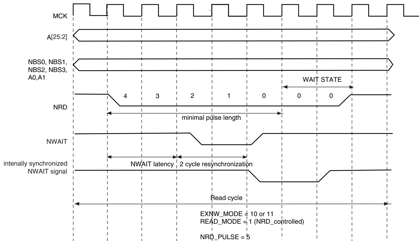
Figure 21-31. NWAIT Latency
