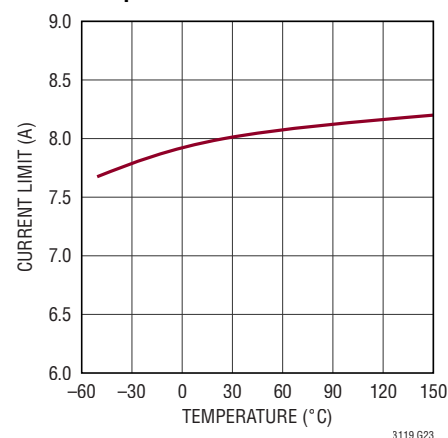
Inductor Current Limit vs Temperature
