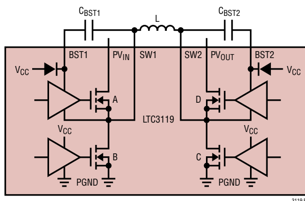
Figure 1. Power Stage Schematic
