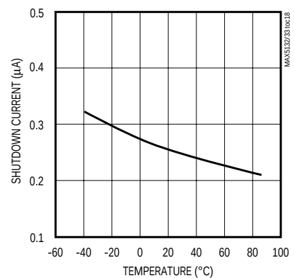
MAX5133 SHUTDOWN CURRENT vs. TEMPERATURE
