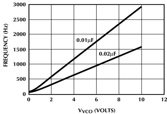
Figure 3. VCO Output Frequency vs. VVCO (Pin 20)
