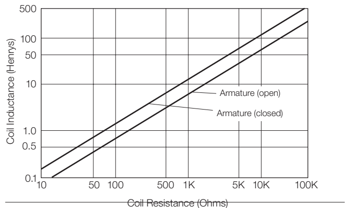
Typical Coil Inductance
