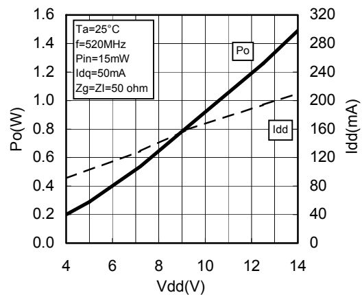
Vdd-Po CHARACTERISTICS
