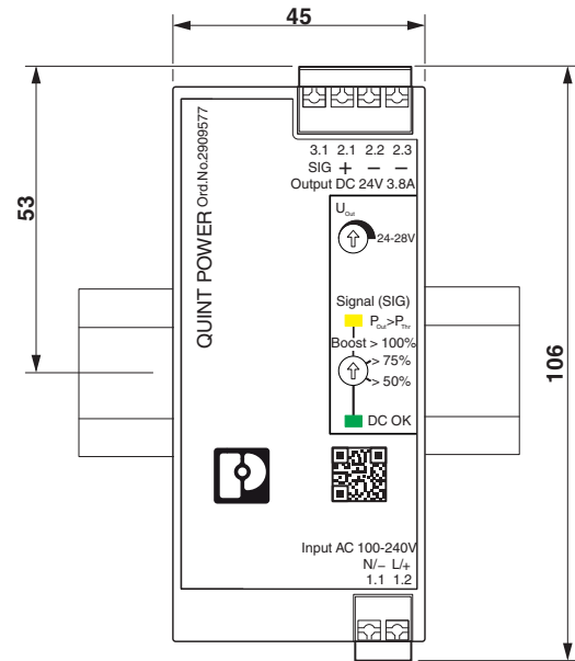
Figure 3 Device dimensions (dimensions in mm)
