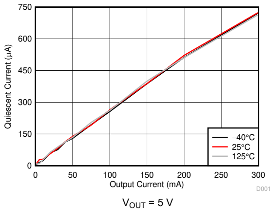
图 6-1. Quiescent Current vs Output Current
