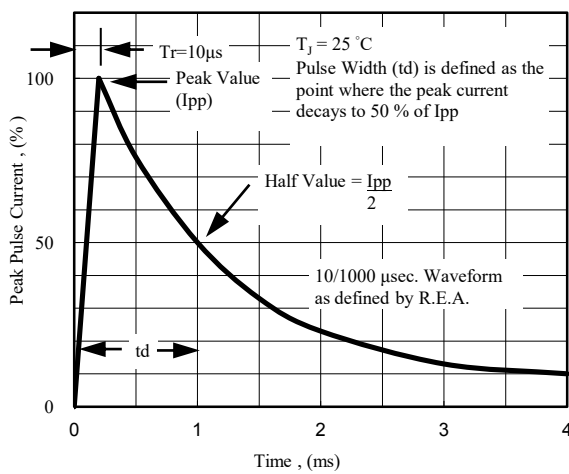
Fig. 5 - Pulse Waveform
