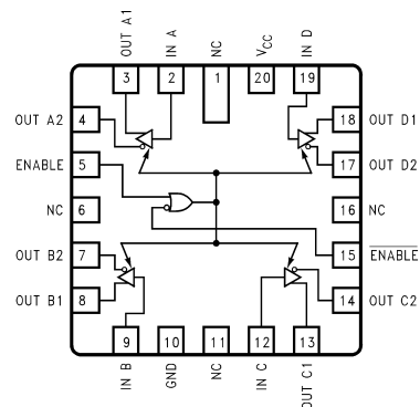
20-Lead Ceramic Leadless Chip Carrier (E)
