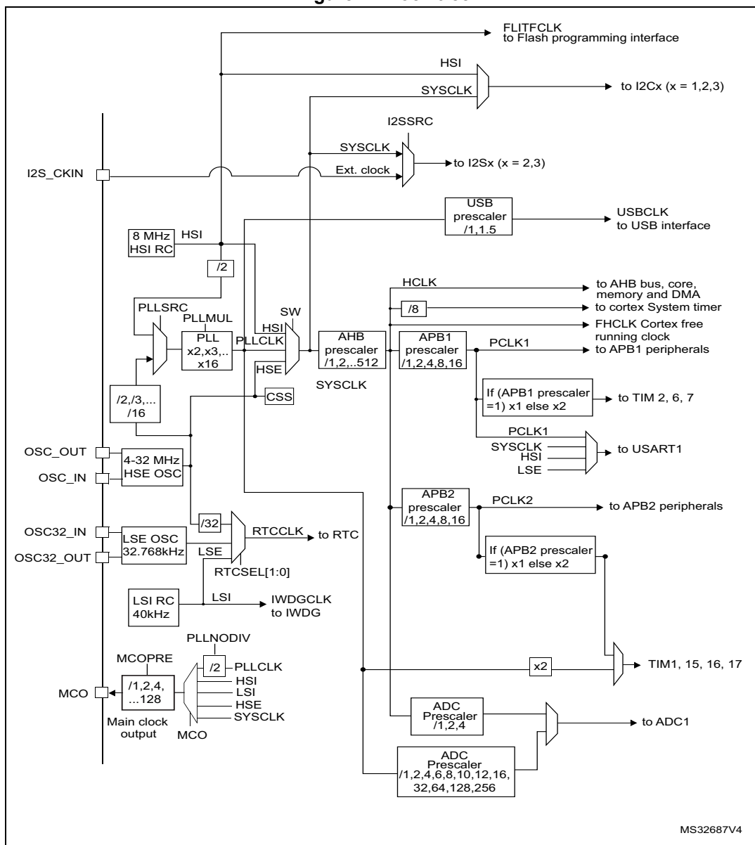
Figure 2. Clock tree
