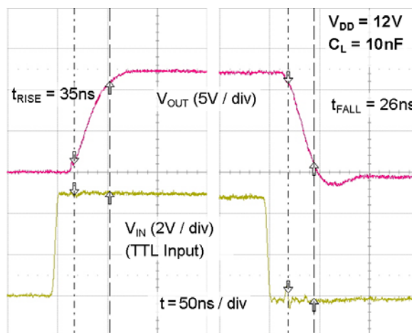
Figure 41. Rise/Fall Waveforms with 10 nF Load
