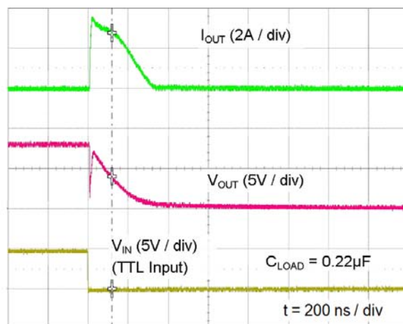
Figure 43. Quasi-Static Sink Current with V_{DD}=12\text{ V}^{(16)}
