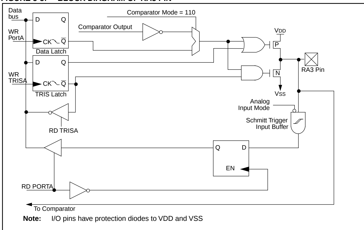
FIGURE 5-3: BLOCK DIAGRAM OF RA3 PIN
