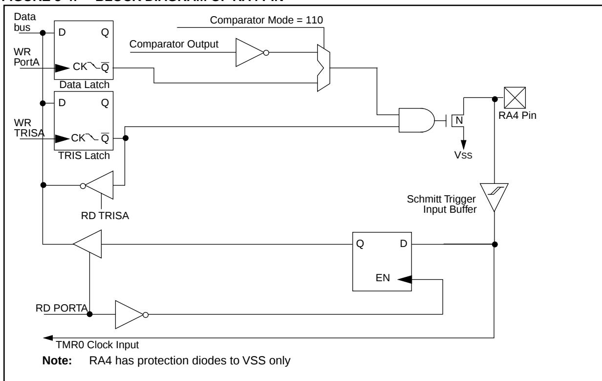
FIGURE 5-4: BLOCK DIAGRAM OF RA4 PIN
