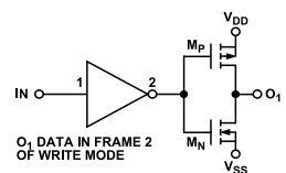
Figure 34. Output Stage of Logic Output, O 1
