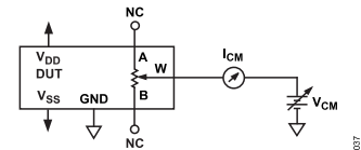
Figure 30. Common-Mode Leakage Current
