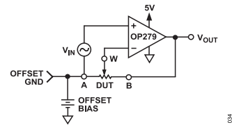
Figure 27. Noninverting Gain
