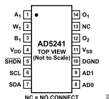
Figure 6. AD5241 Pin Configuration
