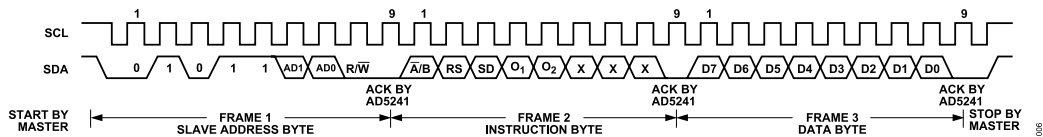
Figure 4. Writing to the RDAC Serial Register
