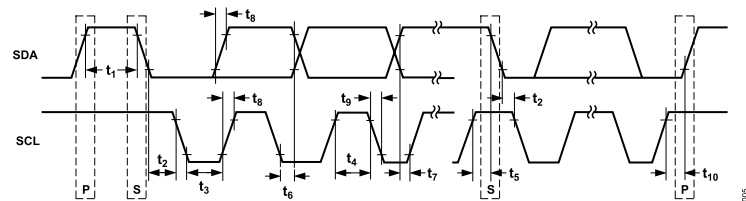
Figure 3. Detail Timing Diagram
