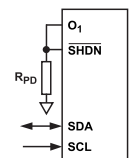
Figure 35. Shutdown by Internal Logic Output, \text{O}_1
