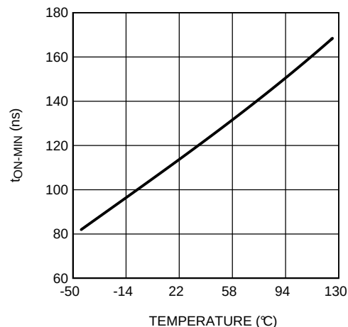
Figure 6. t_{ON-MIN} vs Junction Temperature
