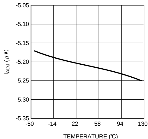
Figure 4. I_{ADJ} vs Junction Temperature
