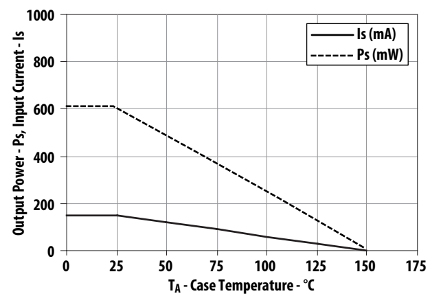
Figure 10: Thermal Derating Curve, Dependence of Safety Limiting Value with Case Temperature per IEC/EN/DIN EN 60747-5-5
