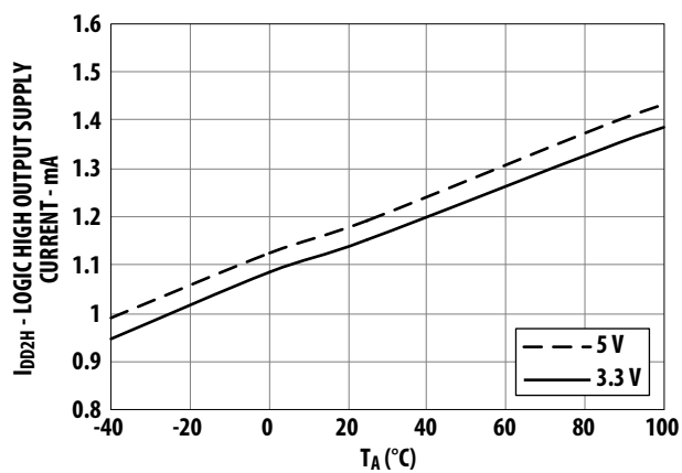
Figure 4: Typical Logic High Output Supply Current vs. Temperature
