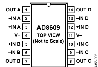
Figure 5. 14-Lead SOIC (R Suffix)
