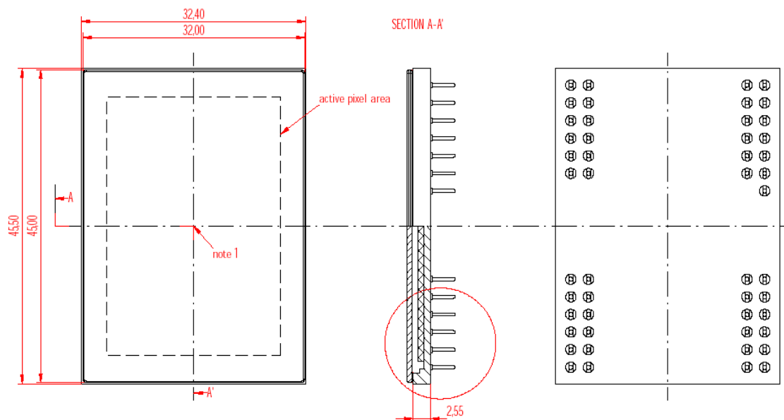
Figure 14. Die Placement
