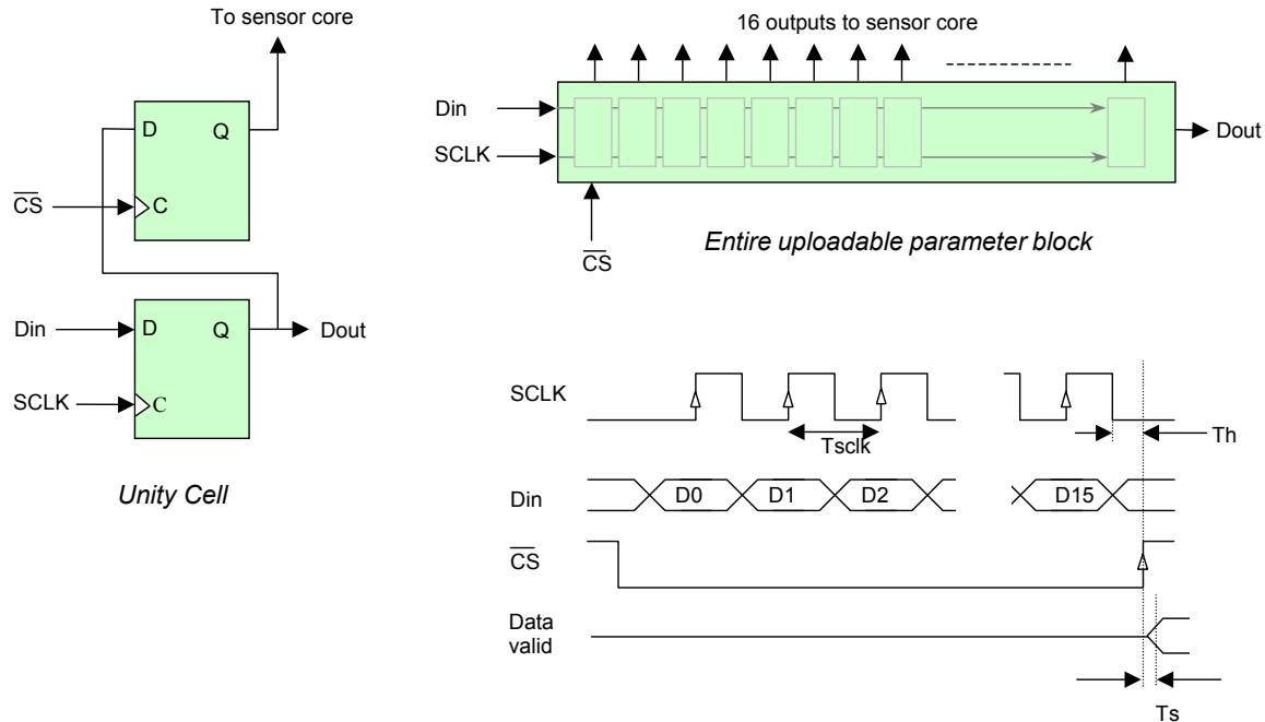
Figure 10. SPI Interface
