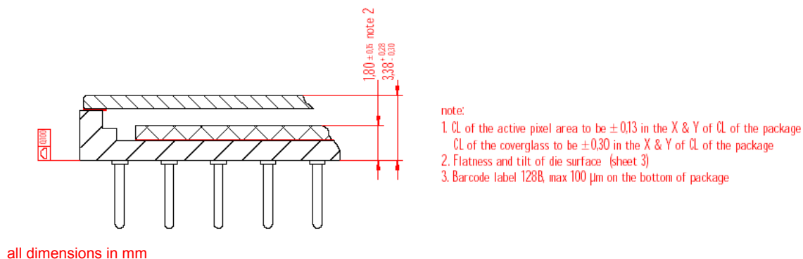
Figure 15. Tolerances
