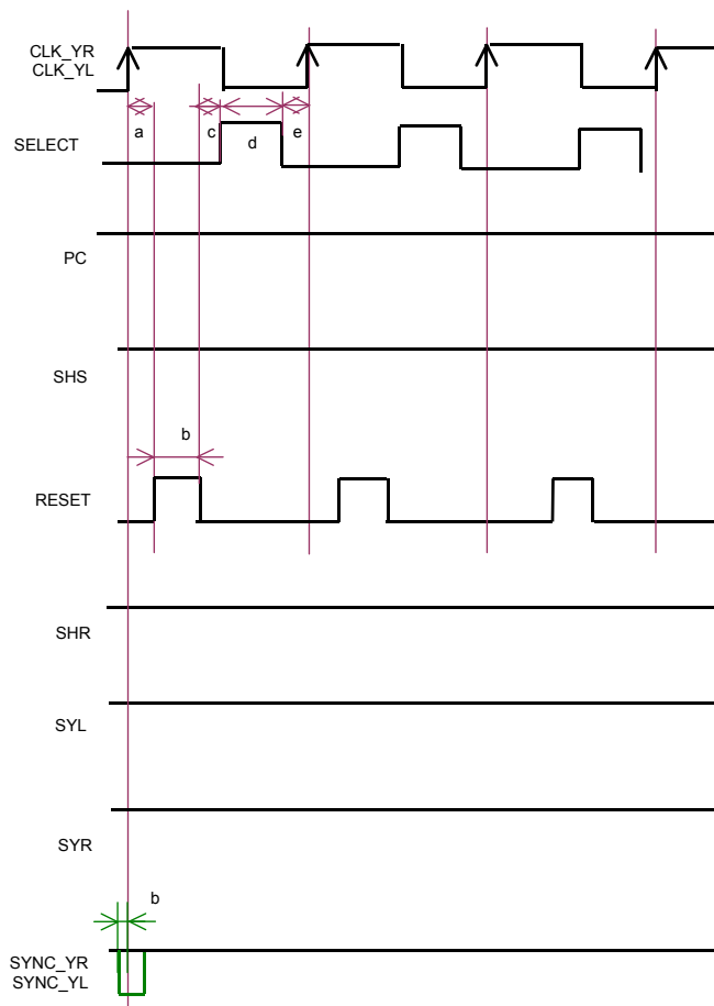
Figure 9. Fast Reset Sequence Timing
