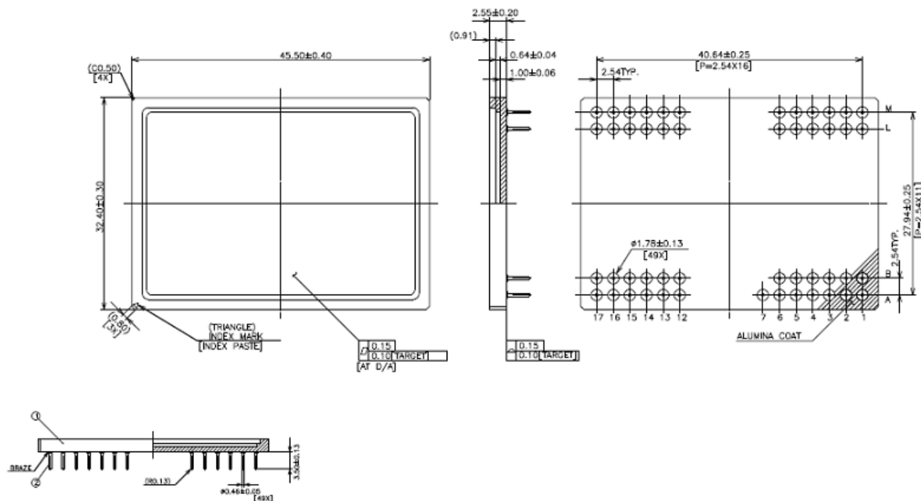
Figure 13. Package Dimensions
