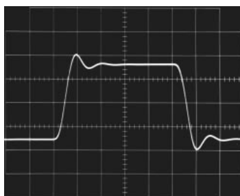
Transient Response
