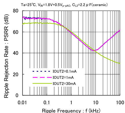
XC6419( V_{OUT2}=0.8V ) VR2
