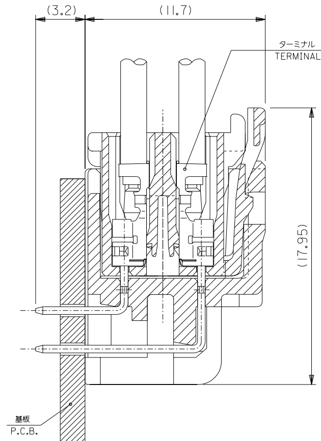
MATED DRAWING (REF.)
