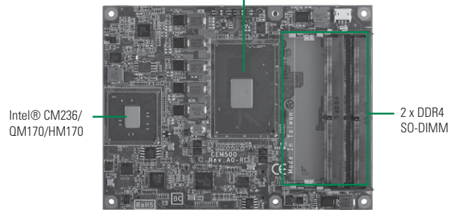
6th Gen. Intel® Xeon® and Core™ Processor
