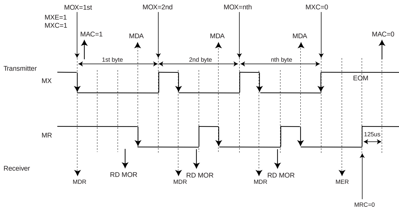
Figure 6-5 Timing chart of general case
