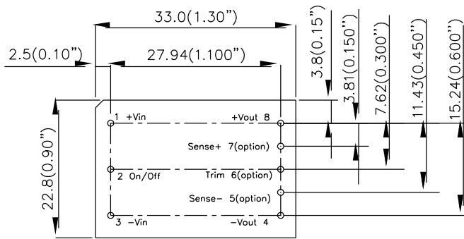
Surface-mount module
