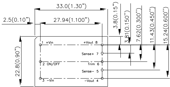
Through-hole module
