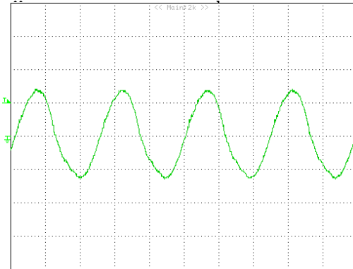
Figure 10: Input Terminal Ripple Current, i_c , at full rated output current and nominal input voltage with 12\mu H source impedance and 33\mu F electrolytic capacitor ( 200\text{ mA/div} , 1\mu s/div )
