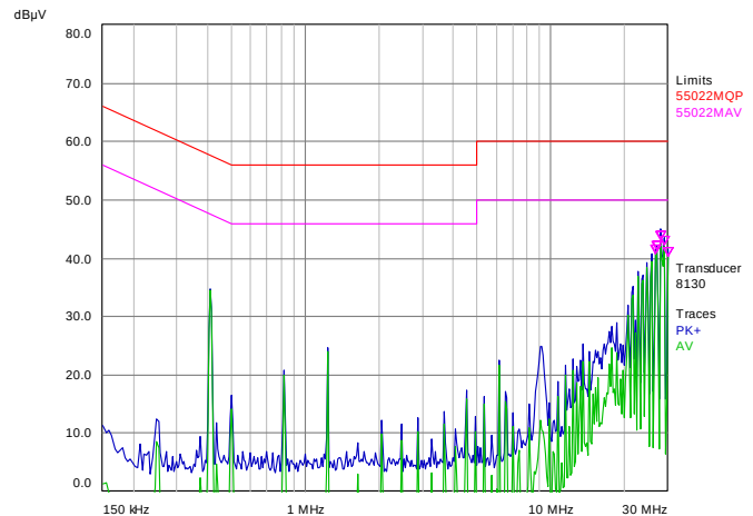
Figure 15 - EMI test
