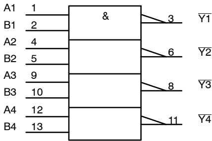
Figure 3. IEC LOGIC DIAGRAM
