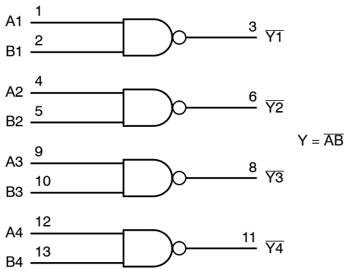
Figure 2. Logic Diagram
