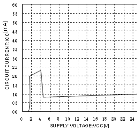
Fig.13 Circuit Current
