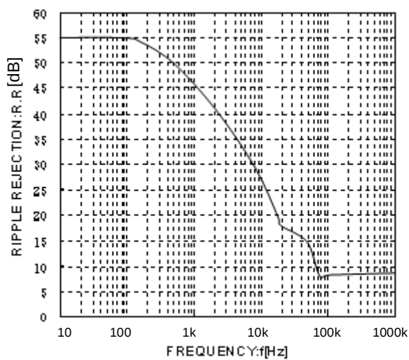
Fig.18 Ripple Rejection Characteristics ( I_o=100mA )
