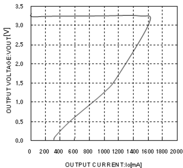
Fig.4 Load Stability
