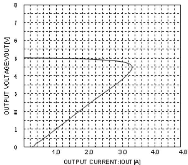
Fig.16 Load Stability
