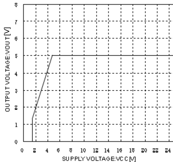
Fig.14 Input Stability
