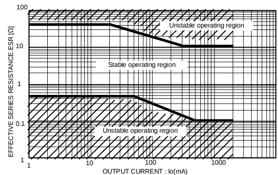
Fig.33: I_o vs. ESR characteristics (BA00DD0XX, 22\mu\text{F} )
