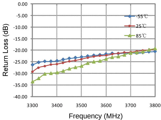
Return Loss (Port 1)
