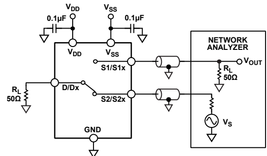
Figure 39. Bandwidth
