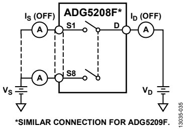
Figure 34. Off Leakage
