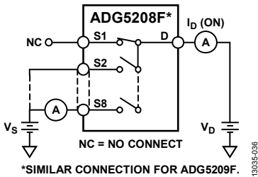
Figure 35. On Leakage
