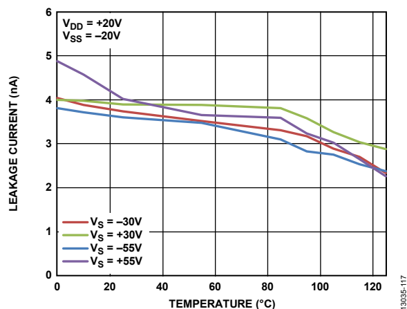
Figure 17. Overvoltage Leakage Current vs. Temperature, \pm 20 V Dual Supply
