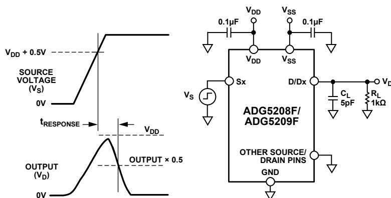
Figure 41. Overvoltage Response Time, t_{RESPONSE}
