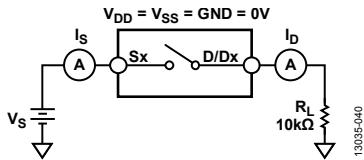
Figure 32. Switch Unpowered Leakage
