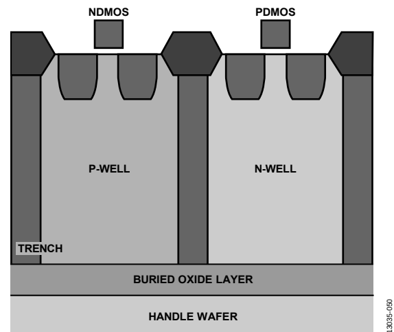
Figure 48. Trench Isolation
