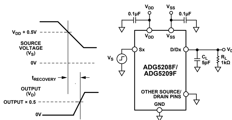
Figure 42. Overvoltage Recovery Time, t_{RECOVERY}
