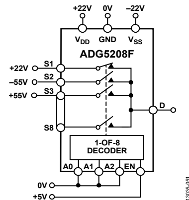
Figure 49. ADG5208F in an Overvoltage Condition
