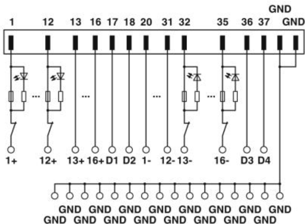
Circuit diagram
