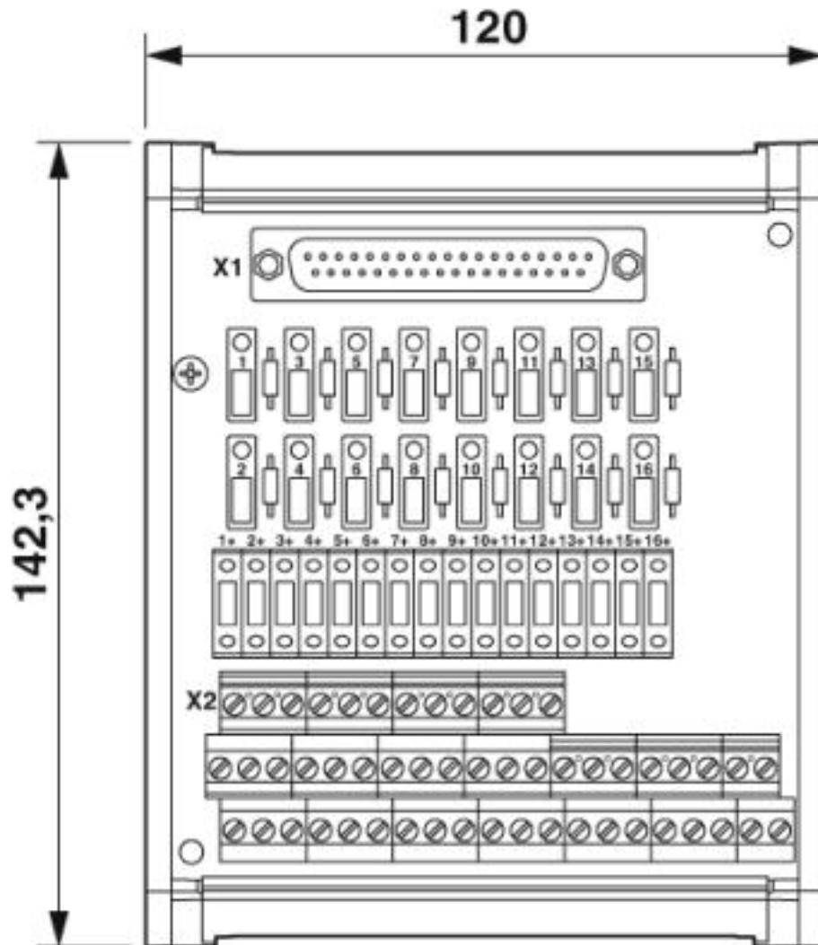
Dimensional drawing
