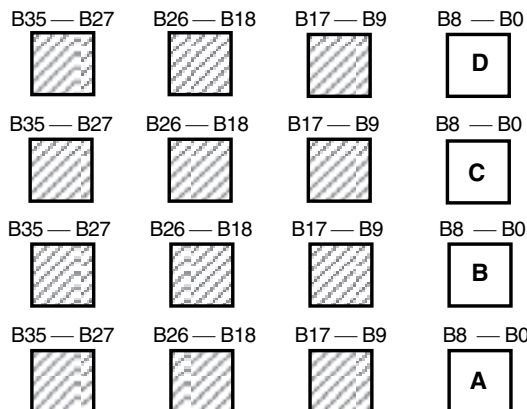
Figure 2. Bus Sizing
