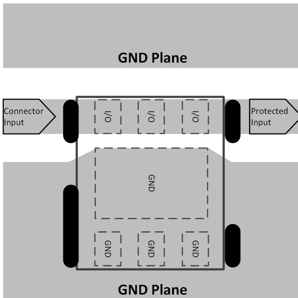
Figure 2. TVS1400 Layout
