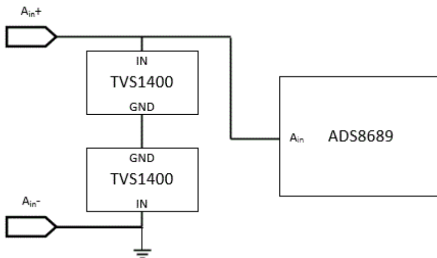
Figure 1. TVS1400 Application Schematic
