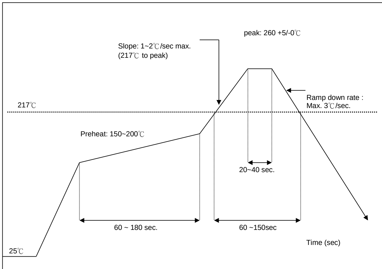
FIGURE 7-5: REFLOW PROFILE
