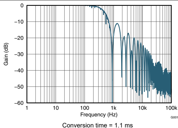
图 7-2. Frequency Response
