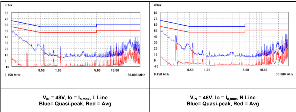
Figure 26. EMC Considerations.
