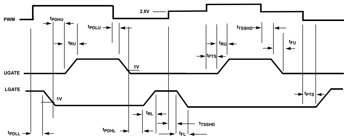
FIGURE 1. TIMING DIAGRAM
