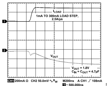
Figure 25. Output Transient Response, C_{OUT} = 4.7 \mu\text{F}
