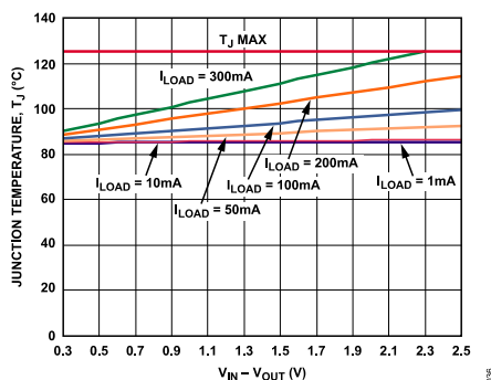
Figure 36. T_A = 85^\circ\text{C}
