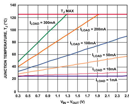
Figure 32. 0 mm 2 of PCB Copper, T_A = 25^\circ\text{C}
