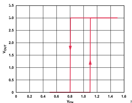
Figure 27. ADP172 Typical EN Pin Operation
