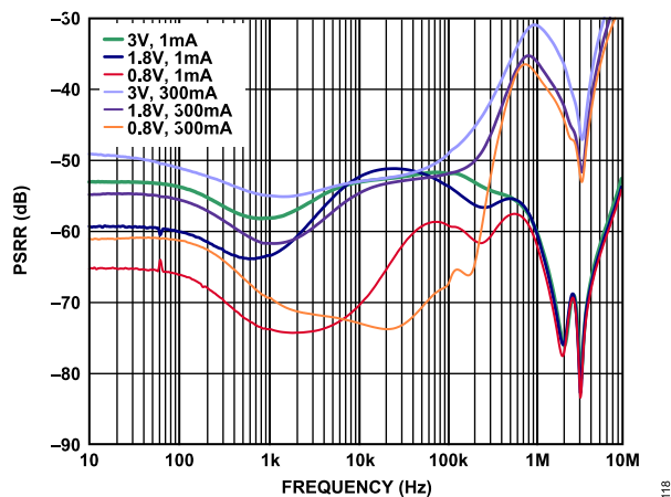
Figure 16. Power Supply Rejection Ratio vs. Frequency, at Various Output Voltages and Load Currents
