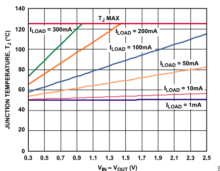
Figure 35. 0 mm 2 of PCB Copper, T_A = 50^\circ\text{C}
