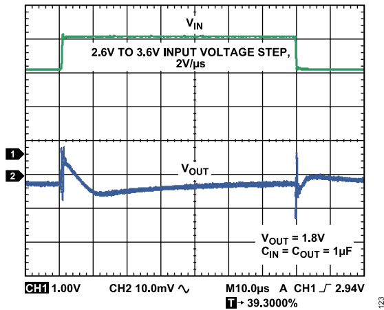
Figure 21. Line Transient Response, Load Current = 1 mA
