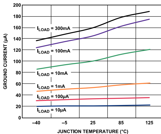
Figure 6. Ground Current vs. Junction Temperature
