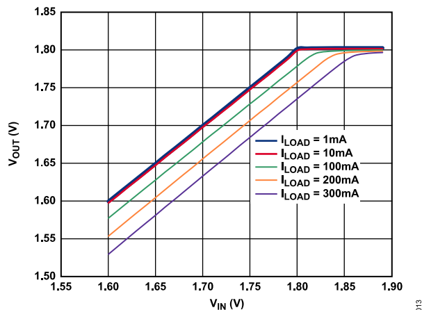
Figure 11. Output Voltage vs. Input Voltage (in Dropout)
