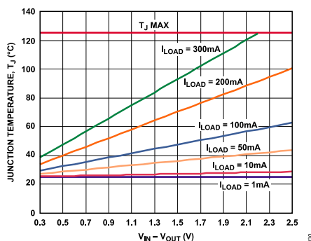
Figure 30. 500 mm 2 of PCB Copper, T_A = 25^\circ\text{C}
