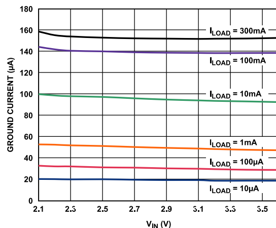
Figure 8. Ground Current vs. Input Voltage
