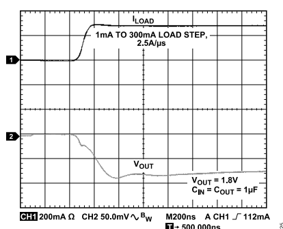
Figure 24. Output Transient Response, C_{OUT} = 1 \mu\text{F}
