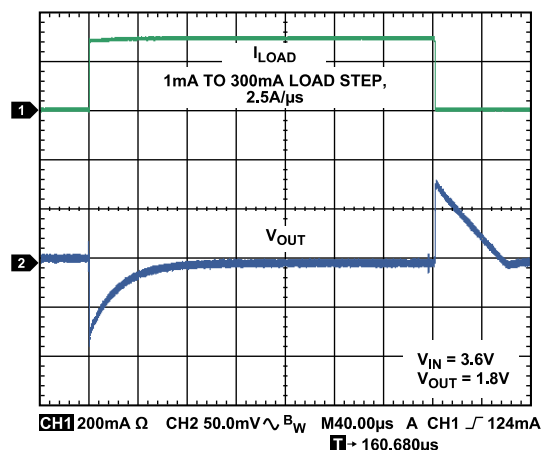
Figure 19. Load Transient Response, C_{IN} and C_{OUT} = 1\text{ }\mu\text{F}
