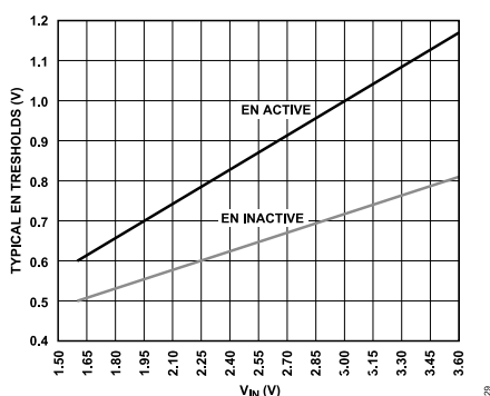
Figure 28. Typical EN Pin Thresholds vs. Input Voltage
