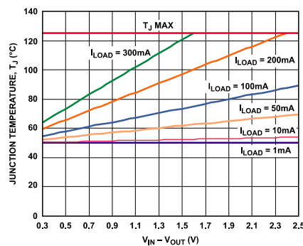
Figure 34. 100 mm 2 of PCB Copper, T_A = 50^\circ\text{C}
