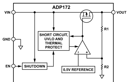
Figure 23. ADP172 Internal Block Diagram
