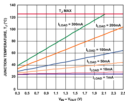
Figure 31. 100 mm 2 of PCB Copper, T_A = 25^\circ\text{C}
