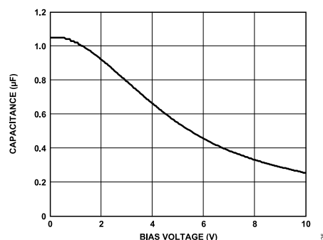
Figure 26. Capacitance vs. Bias Voltage Characteristics
