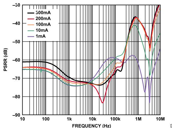
Figure 13. Power Supply Rejection Ratio vs. Frequency, V_{OUT} = 0.8\text{ V}
