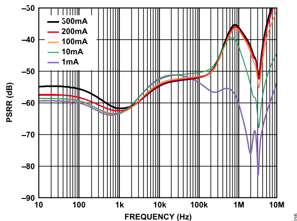
Figure 14. Power Supply Rejection Ratio vs. Frequency, V_{OUT} = 1.8\text{ V}
