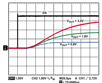
Figure 29. Typical Start-Up Time
