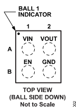
Figure 2. Pin Configuration
