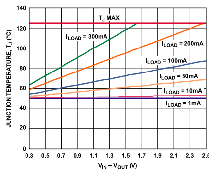
Figure 33. 500 mm 2 of PCB Copper, T_A = 50^\circ\text{C}
