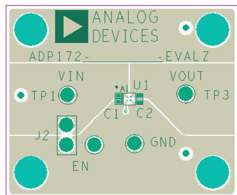
Figure 37. Example ADP172 PCB Layout
