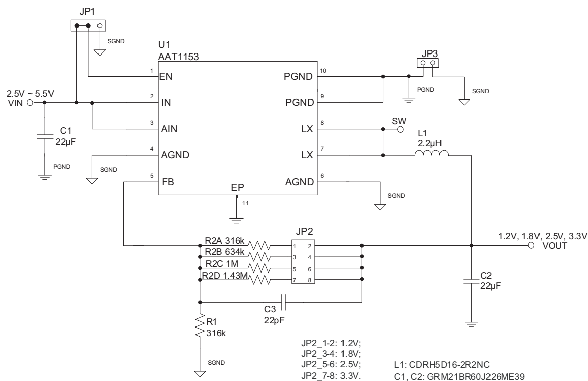
Figure 2: AAT1153 Recommended Evaluation Board Schematic.
