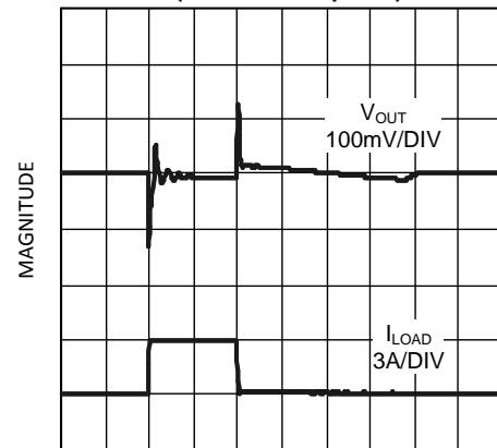
Load Transient Response (Tantalum 100 \mu\text{F}/3\text{A} )
