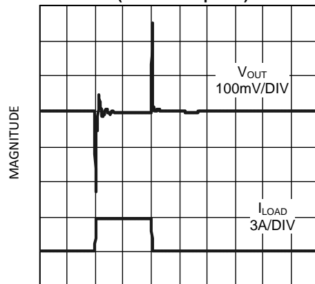
Load Transient Response (SANYO 150 \mu\text{F}/3\text{A} )
