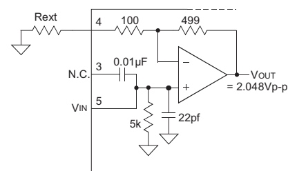
Figure 2c. Non-inverting Mode
