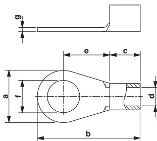
Dimensioned drawing
