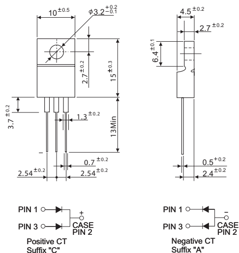
TO-220F15
