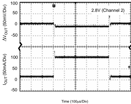
Figure 39. Load Transient
