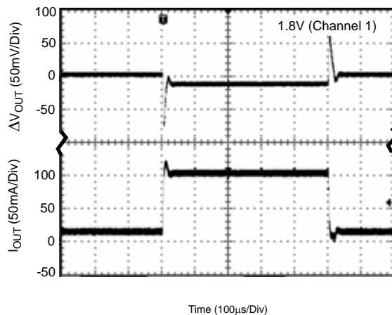
Figure 37. Load Transient
