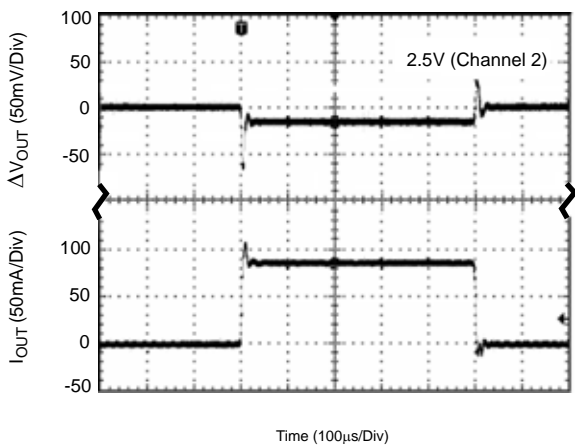
Figure 38. Load Transient
