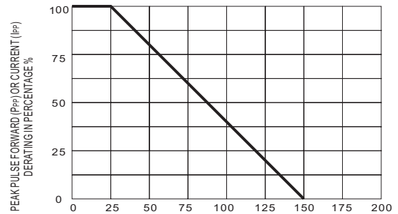
Fig.2 DERATING CURVE
