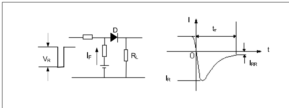
Diagram of Circuit and Testing Wave form of Reverse Recovery Time t_r
