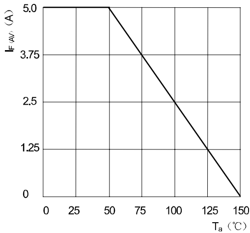
I_{F(AV)} - T_a Derating
