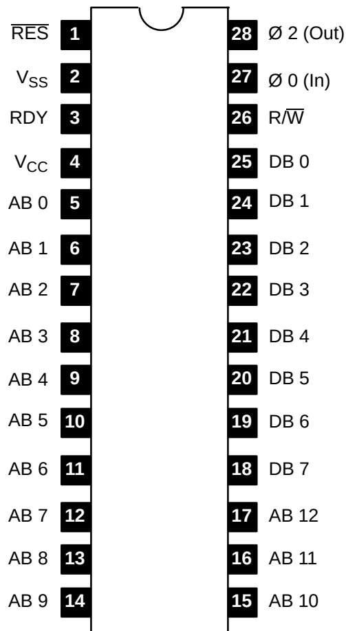
Pin Connection Diagram
