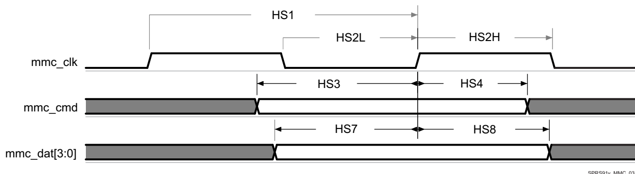
Figure 7-41. MMC/SD/SDIOj in - High Speed - Receiver Mode
