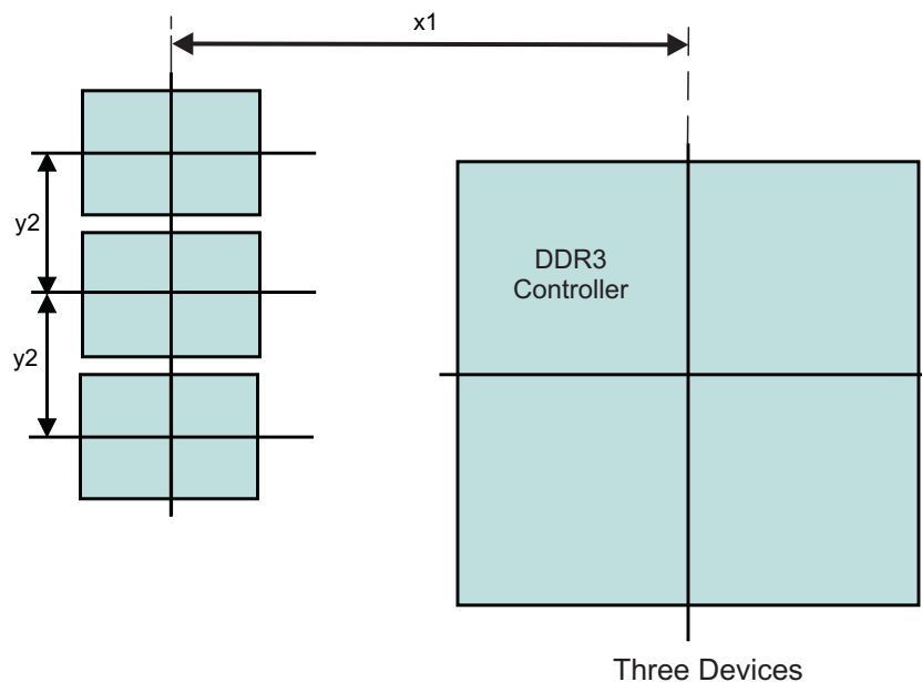
Figure 8-47. Placement Specifications
