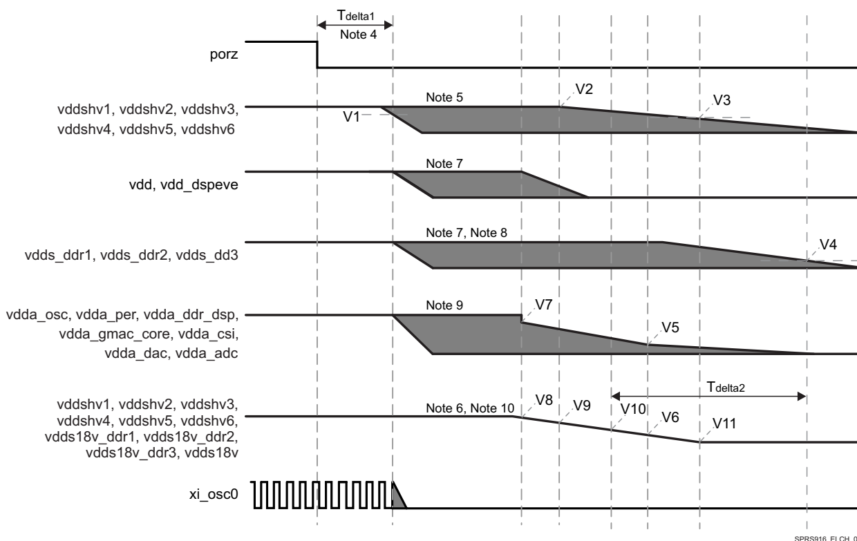
Figure 5-6. Abrupt Power-Down Sequencing (1)
