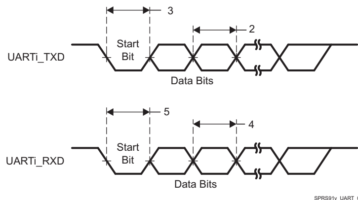
Figure 7-25. UART Timing
