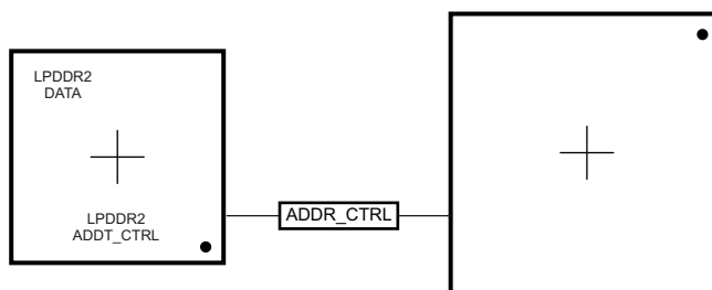
Figure 8-35. ADDR_CTRL Signals Routing
