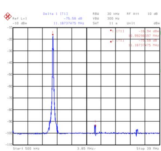
FIGURE 4. GSM AT 11MHz, 78MSPS CLOCK (75dBc - NYQUIST, 9dB PAD)
