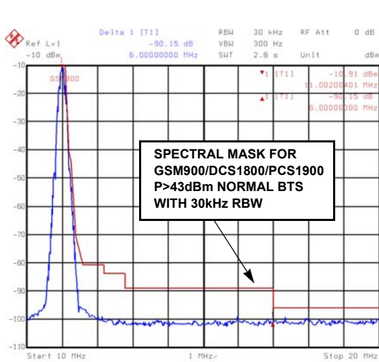
FIGURE 3. GSM AT 11MHz, 78MSPS CLOCK (90+dBc @ \Delta f = +6 MHz, 3dB PAD)
