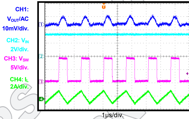
Steady State I_{OUT} = 0A , FCCM
