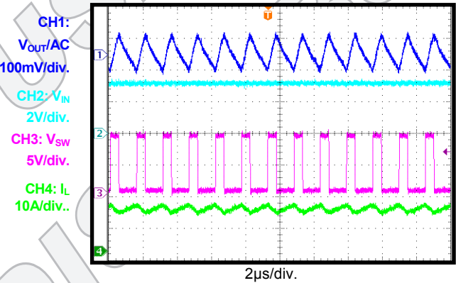
Steady State I_{OUT} = 3.5A
