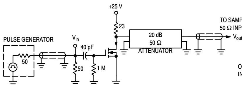
Figure 1. Switching Test Circuit
