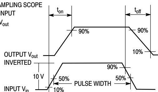
Figure 2. Switching Waveforms
