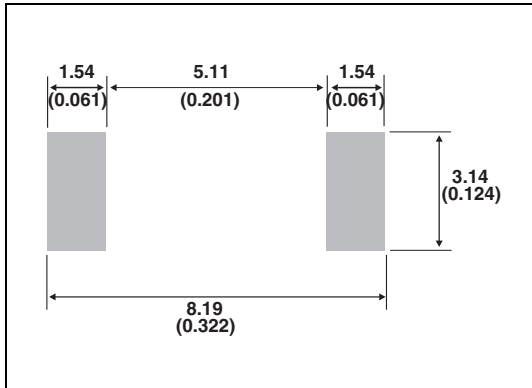
Figure 17. SMC footprint dimensions in mm (inches)
